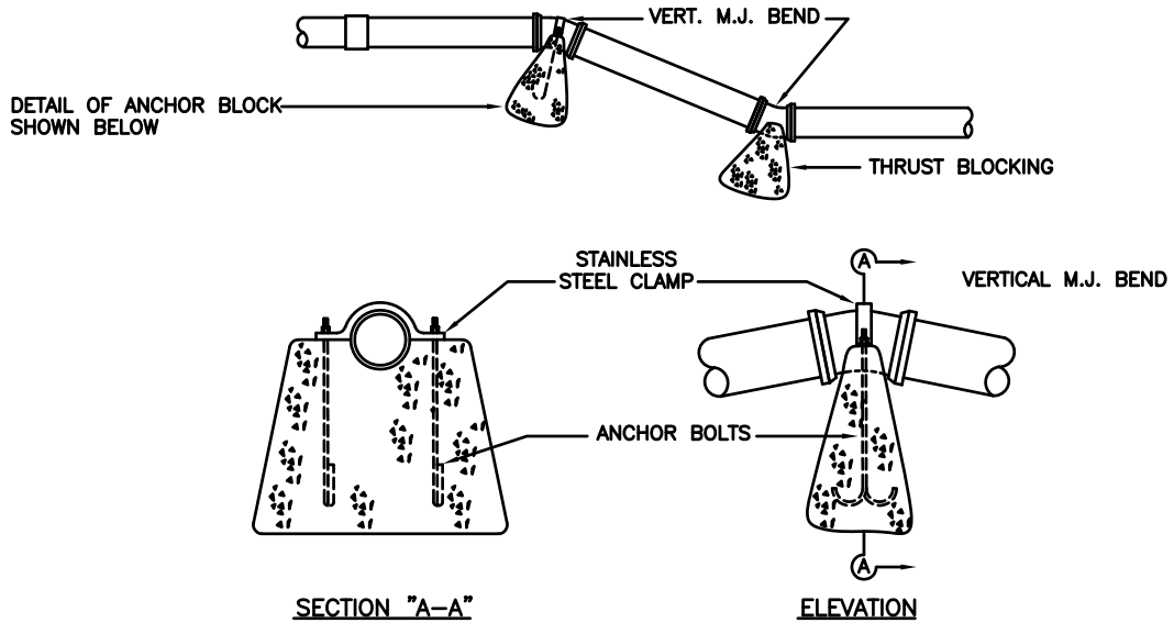
TYPICAL CONCRETE ANCHOR BLOCK FOR VERTICAL BEND
