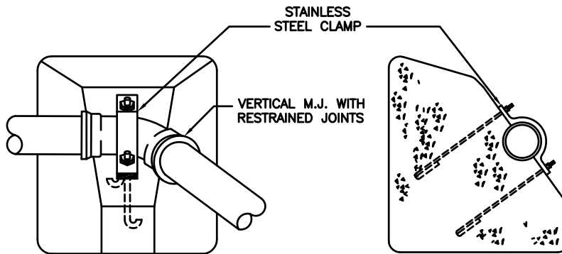
TYPICAL CONCRETE ANCHOR BLOCK FOR COMBINATION HORIZONTAL - VERTICAL BEND
