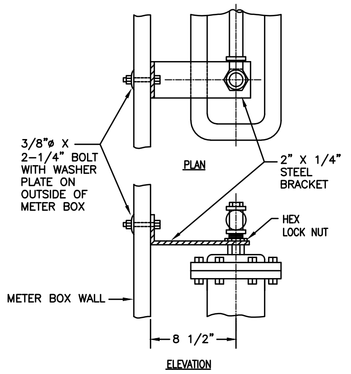
BRACKET DETAIL
