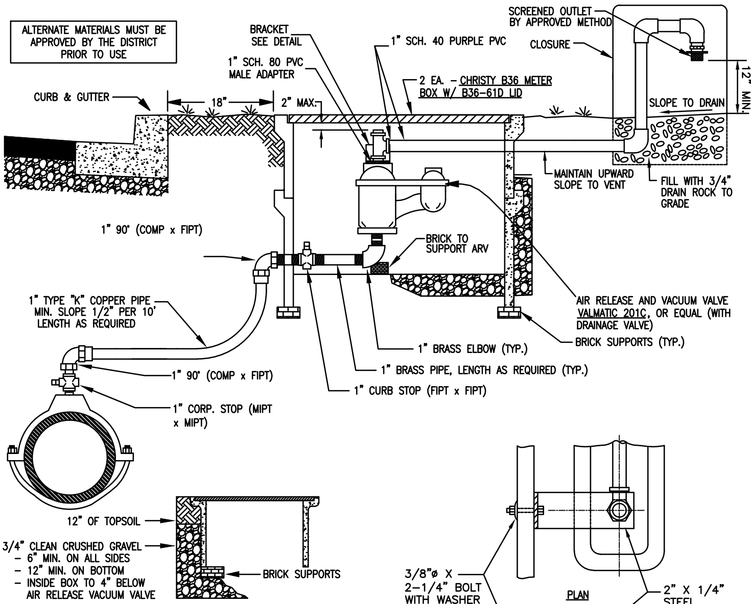
DETAIL - BOX INSTALLATION
